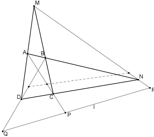
Figure 1. The Newton property
